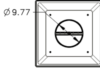
10" HT-2X2-SPL10
